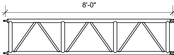
Top / Plan
