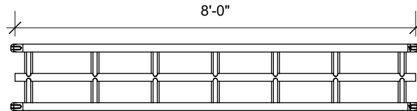
Top / Plan
